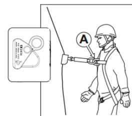
Connection of the device to a safety harness
